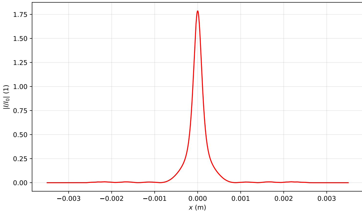
Intensity profile I(x, y = 0, z = 0.955)/I_0 , P_{in}=4.0P_{cr} , artificial time
